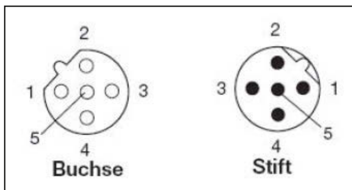
Profibus connector M12, 5- pole, B- coded
